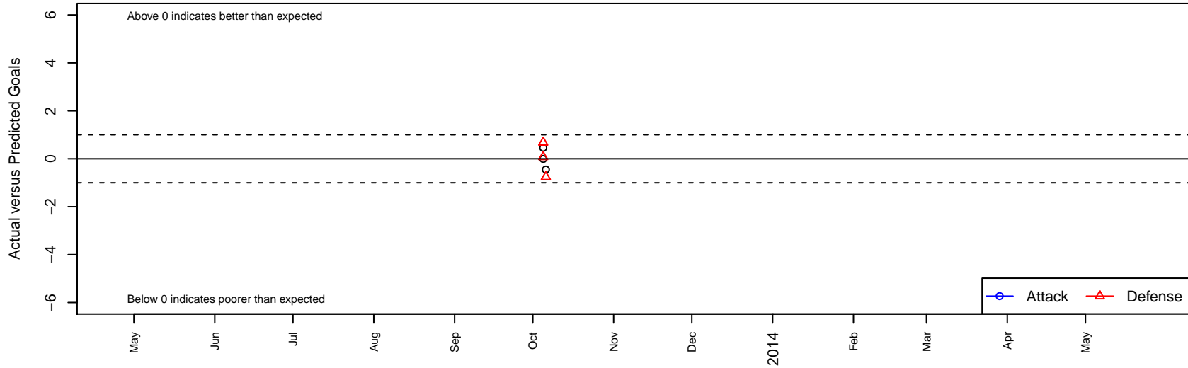
PVSC United Thunder G01 Dots are actual minus expected GF (blue circles) and GA (red triangles). Blue line is smoothed change in attack strength. Red is smoothed change in defense strength.
